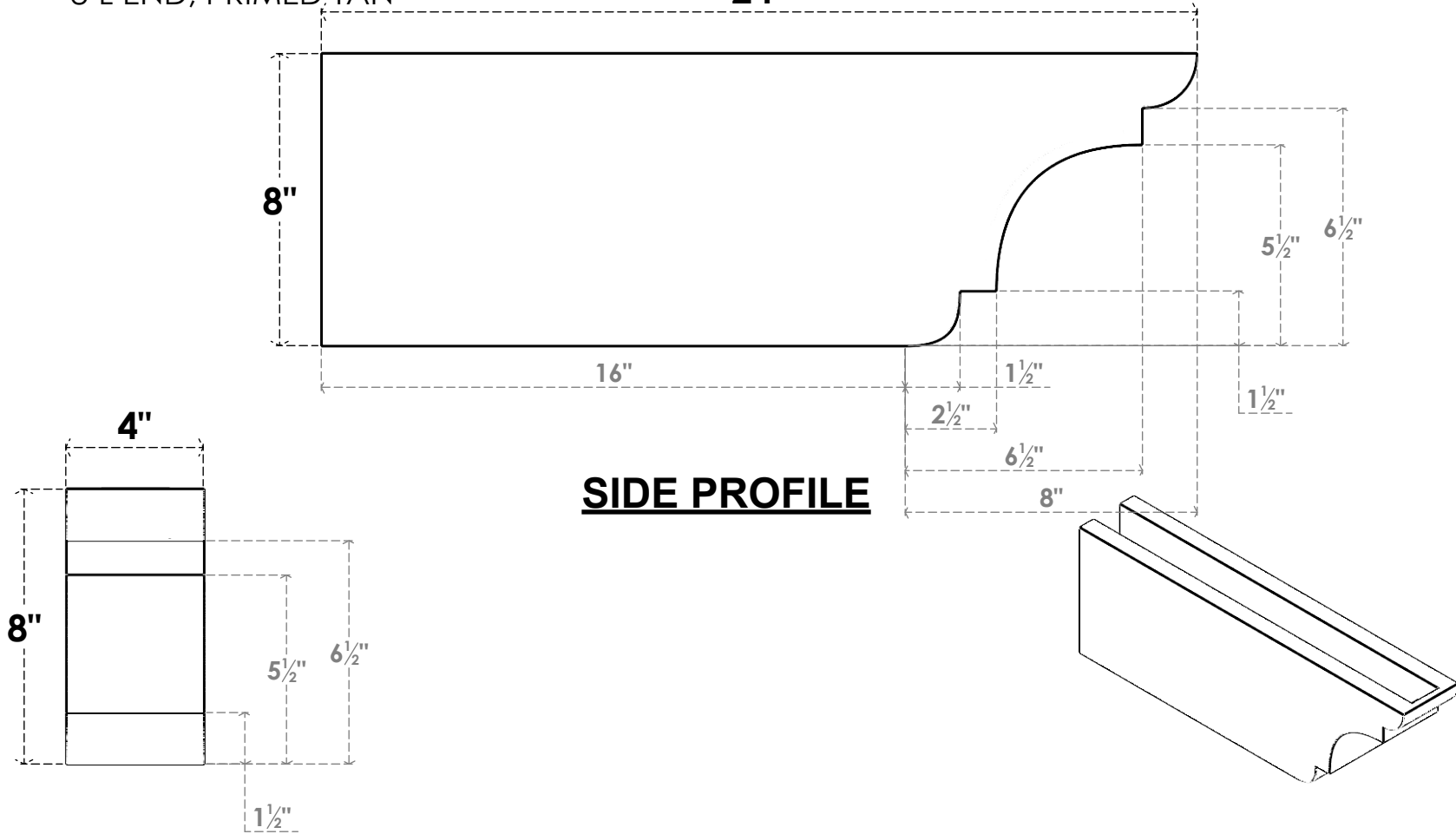
FRONT PROFILE
